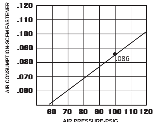
AIR CONSUMPTION CHART
